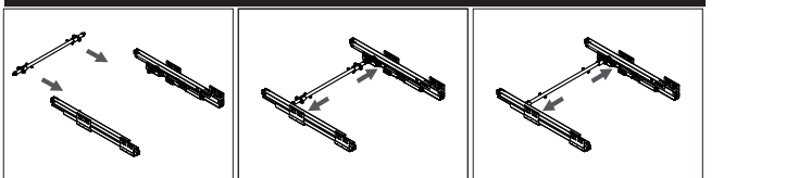
Cut the rod Snap the rod into push-open device on the slide Screw on and finish
