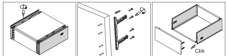
Fix screws Front assembly
