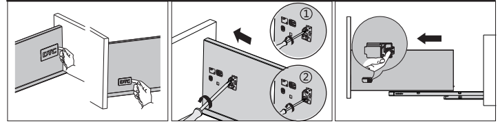
Tip up the cover and pull out Turn screw driver to release the drawer front Lift the release handle and Pull out the drawer
