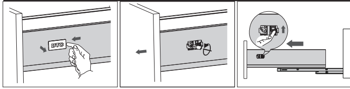
Tip up the cover and pull out Turn screw driver to release the drawer front Lift the release handle and Pull out the drawer
