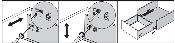
Left&right adjustment Up&down adjustment Slide into the cabinet
