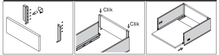
Back assembly
