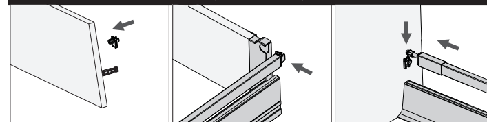
Front assembly
