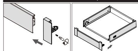
Front assembly
