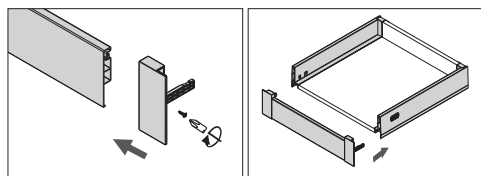
Front assembly
