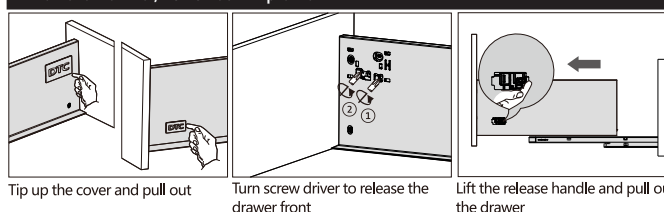
Lift the release handle and pull out the drawer
