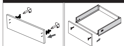
Front assembly
