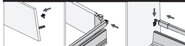
Front assembly
