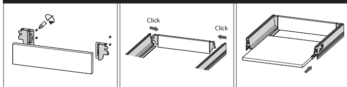
Back assembly
