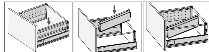
Side assembly
